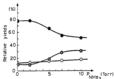
Figure 8. Relative yields of isomeric methylpyrroles 2-4 from pyrrole 1 in the competition experiments, at 760 torr, as a function of the partial pressure NMe_3 ( P_{NMe_3} ): (●) 3-methylpyrrole (4); (○) 2-methylpyrrole (3); (○) N -methylpyrrole (2).
