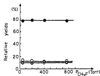
Figure 7. Relative yields of isomeric methylpyrroles 2–4 from pyrrole 1 in the competition experiments, as a function of the total pressure ( P_{\text{CH}_3\text{F}} ) of the system, in the absence of NMe 3 : (●) 3-methylpyrrole ( 4 ); (⊙) 2-methylpyrrole ( 3 ); (○) N -methylpyrrole ( 2 ).
