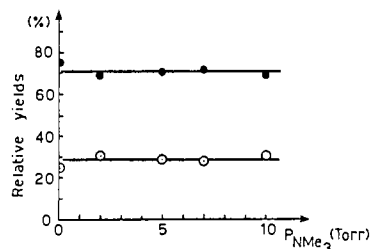
Figure 10. Relative yields of isomeric dimethylpyrroles 5-6 from CH_3FCH_3^+ attack on N -methylpyrrole (2), at 760 torr, as a function of the partial pressure of NMe_3 ( P_{NMe_3} ): (●) 1,3-dimethylpyrrole (6); (○) 1,2-dimethylpyrrole (5).
