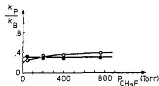
Figure 3. Dependence of the apparent k_p/k_B ratios (see text) on the total pressure of the competition systems: (○) pyrrole 1/benzene; (●) N -methylpyrrole (2)/benzene.
