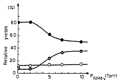
Figure 6. Relative yields of isomeric methylpyrroles 2–4 from CH 3FCH 3 + attack on pyrrole 1 , at 760 torr, as a function of the partial pressure of NMe 3 ( P_{\text{NMe}_3} ): (●) 3-methylpyrrole ( 4 ); (⊙) 2-methylpyrrole ( 3 ); (○) N -methylpyrrole ( 2 ).
