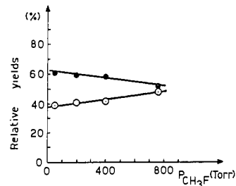
Figure 11. Relative yields of isomeric dimethylpyrroles 5-6 from N -methylpyrrole (2) in the competition experiments, as a function of the total pressure ( P_{CH_3F} ) of the system, in the absence of NMe_3 : (●) 1,3-dimethylpyrrole (6); (○) 1,2-dimethylpyrrole (5).
