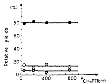
Figure 5. Relative yields of isomeric methylpyrroles 2–4 from CH 3FCH 3 + attack on pyrrole 1 as a function of the total pressure ( P_{\text{CH}_3\text{F}} ) of the system, in the absence of NMe 3 : (●) 3-methylpyrrole ( 4 ); (⊙) 2-methylpyrrole ( 3 ); (○) N -methylpyrrole ( 2 ).
