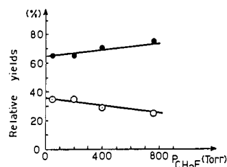
Figure 9. Relative yields of isomeric dimethylpyrroles 5-6 from CH_3FCH_3^+ attack on N -methylpyrrole (2) as a function of the total pressure ( P_{CH_3F} ) of the system, in the absence of NMe_3 : (●) 1,3-dimethylpyrrole (6); (○) 1,2-dimethylpyrrole (5).
